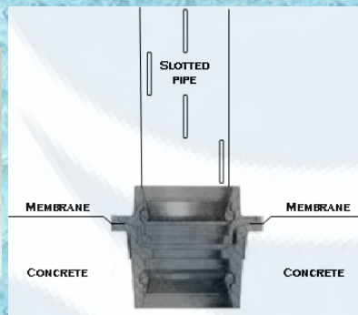
PLANTER BOX DRAIN 100MM SLOTTED PVC
